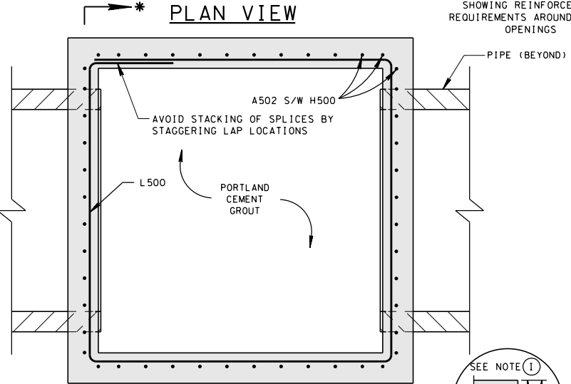
SECTION E-E
